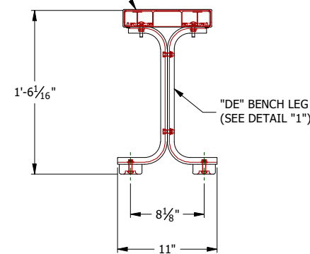
RUBBER FOOT PAD OPTION SEE DETAIL "2"
