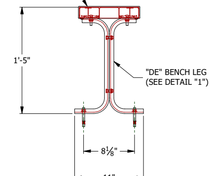
CONCRETE ANCHORED OPTION SEE DETAIL "3"
